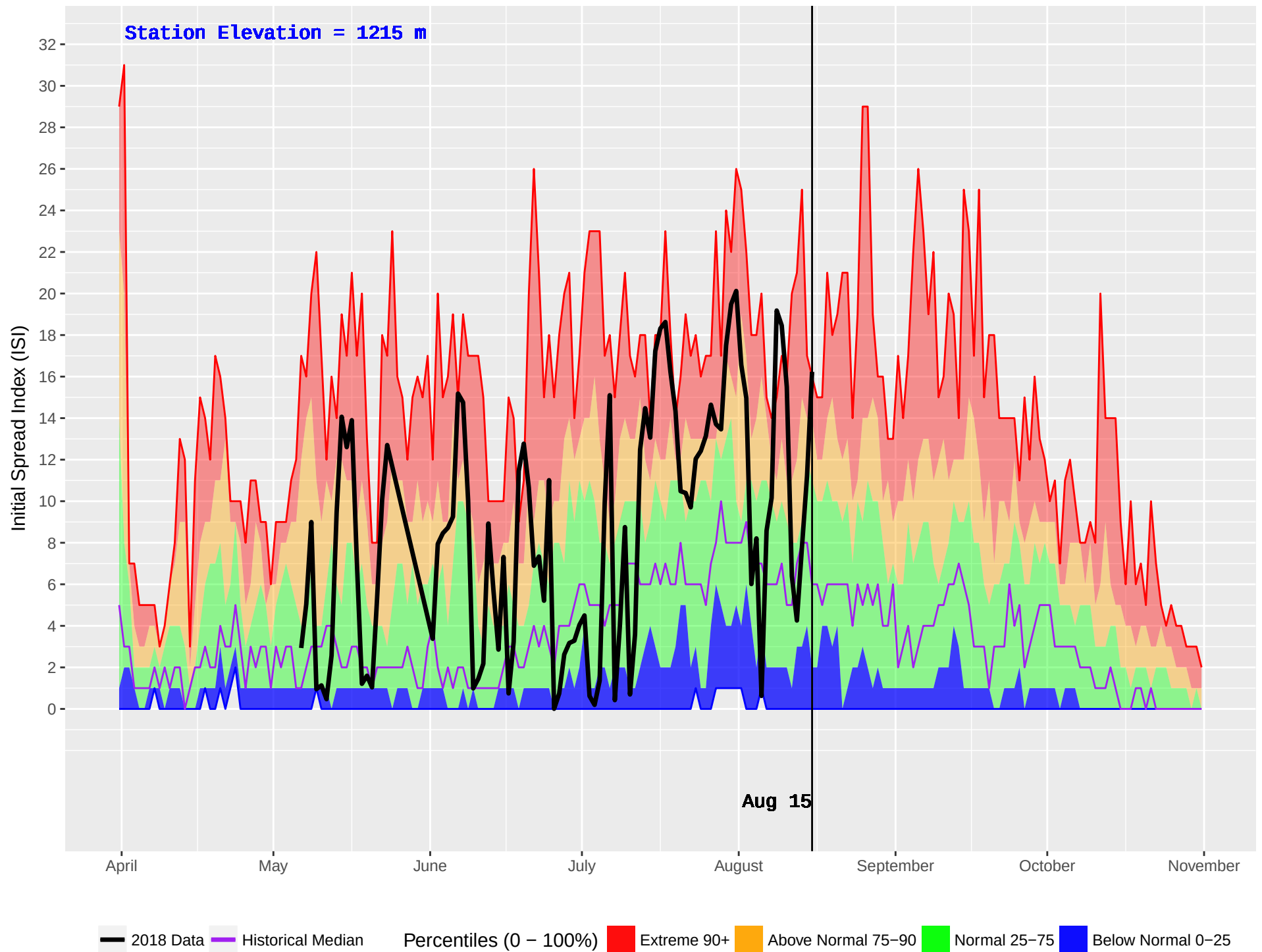
ALLISON PASS (317) : Historical (1987–2016) and Current (2018) Daily Initial Spread Index (ISI)
