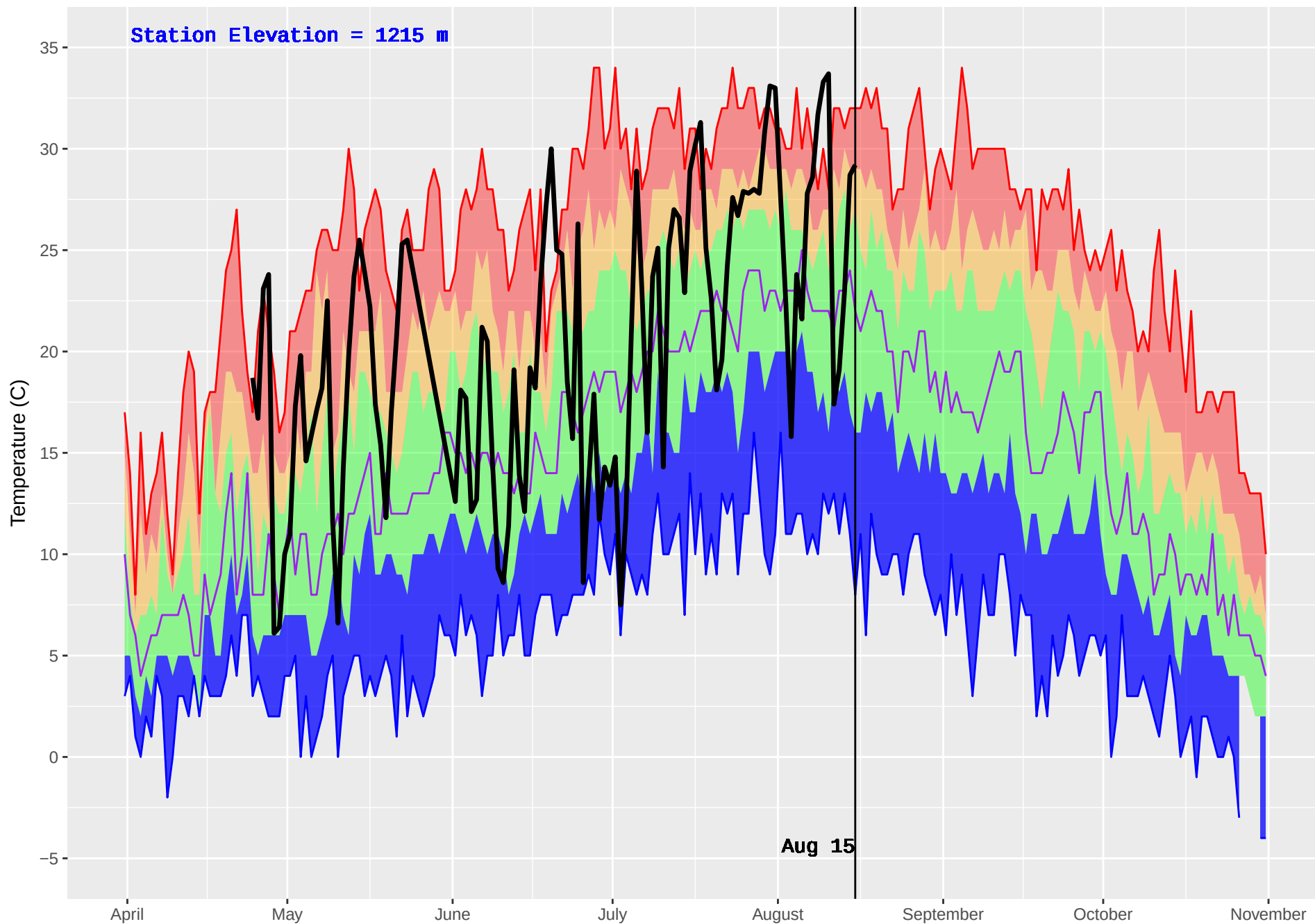
ALLISON PASS (317) : Historical (1987–2016) and Current (2018) Daily Temperature
