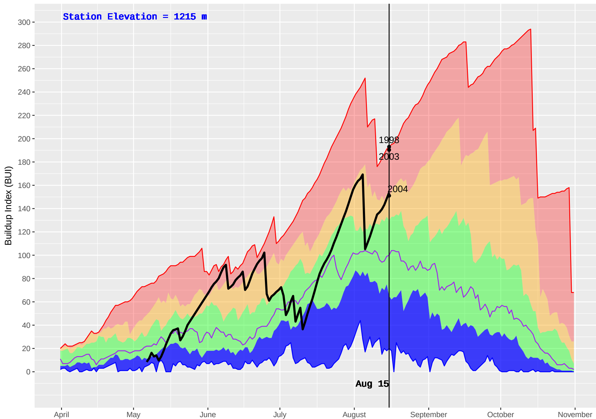
ALLISON PASS (317) : Historical (1987–2016) and Current (2018) Daily Buildup Index (BUI)
